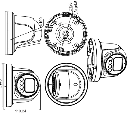
Figure 2-4 Dimensions Unit: mm
